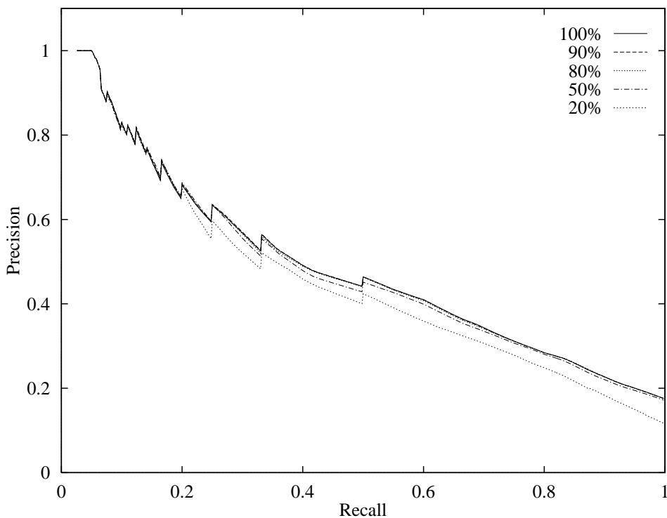
Figure 5: Average precision vs. recall when evaluation is stopped after a fixed percentage of features.
